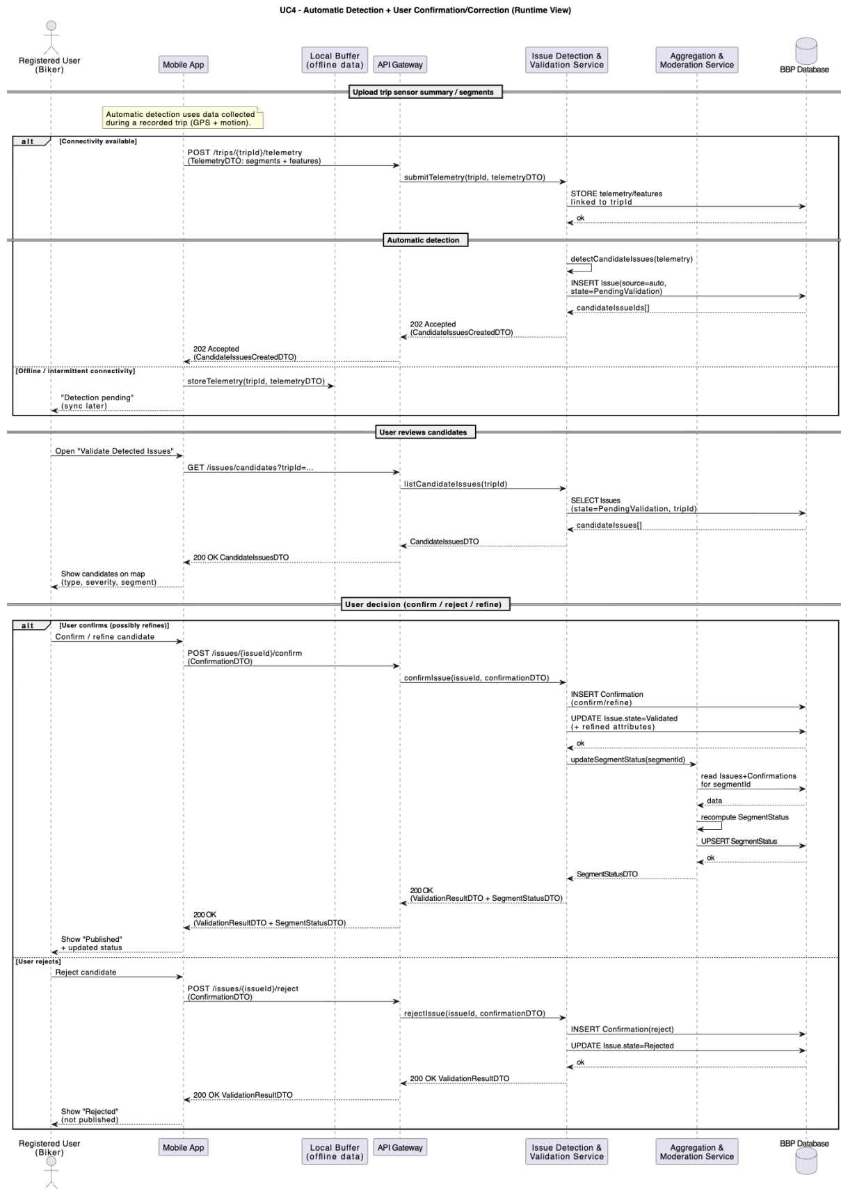
Figure 7: Runtime View of UC4
