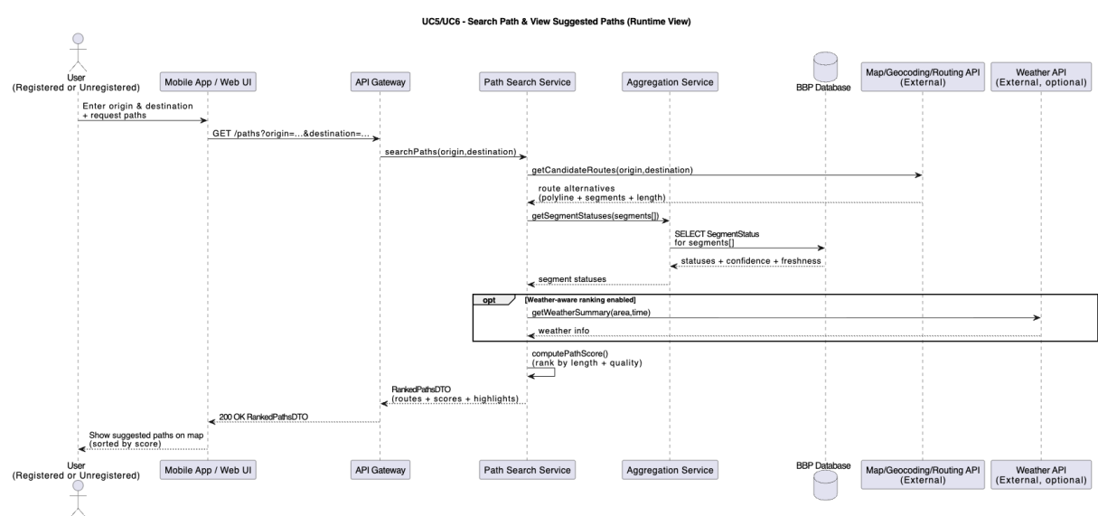
Figure 4: Runtime View of UC5+UC6
