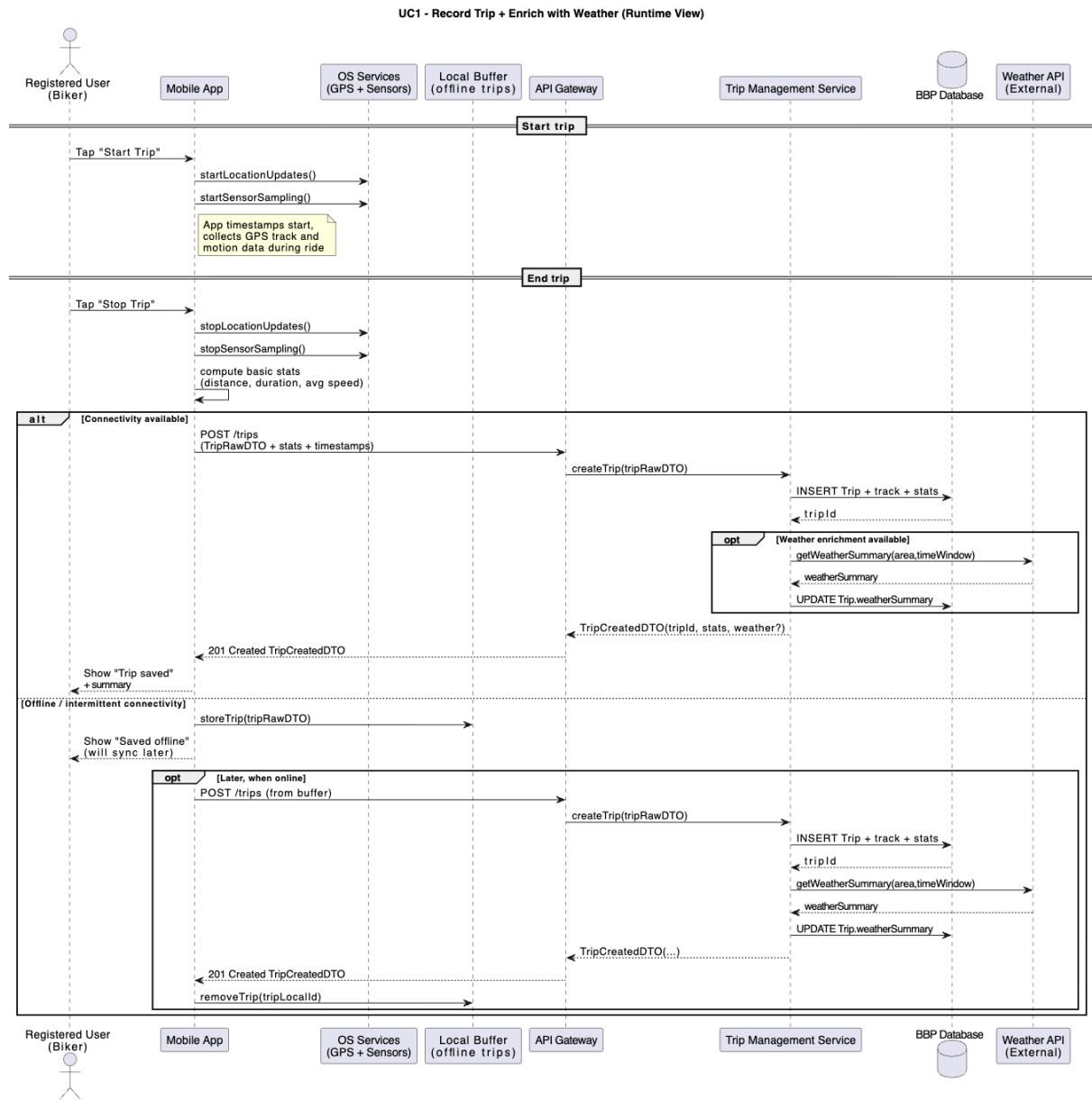
Figure 5: Runtime View of UC1
