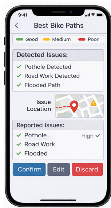
Figure 12: Interface for confirmation of automatically detected issues
