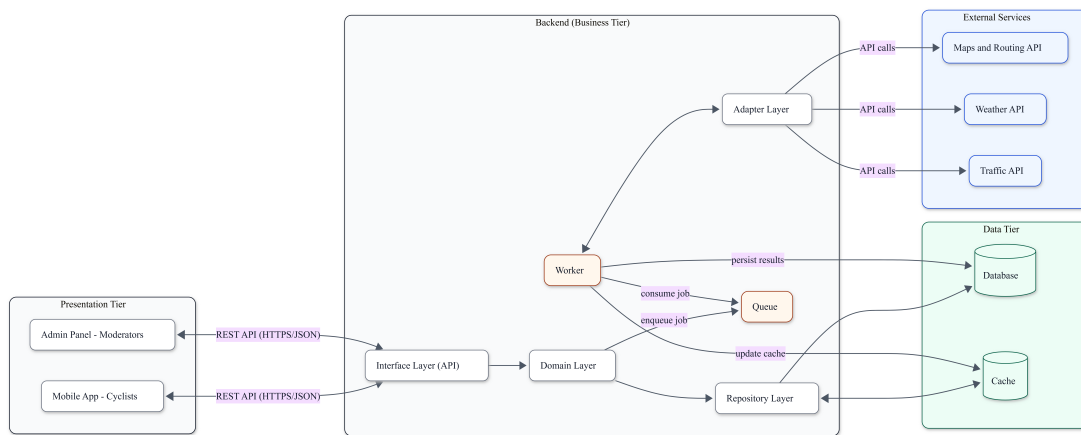
Figure 1: Component interactions in the BBP architecture
