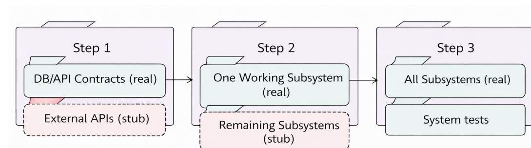
Figure 14: Incremental integration strategy with progressive replacement of stubs.
