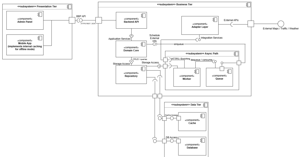
Figure 2: BBP component diagram (annotated)
