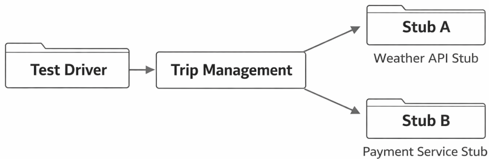
Figure 13: Component testing using a test driver and stubs.
