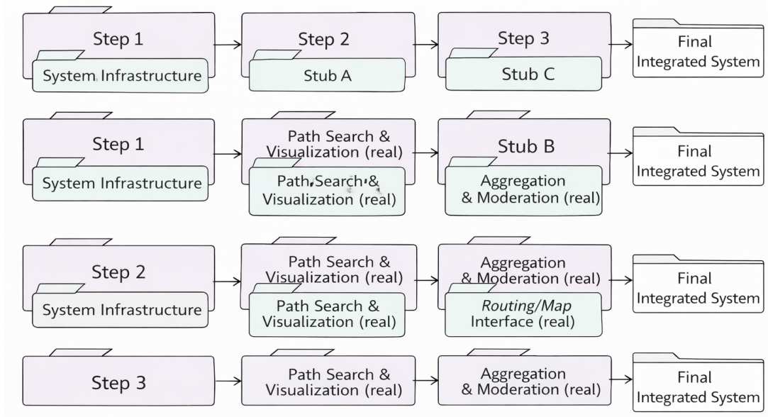
Figure 15: Thread-based integration of the Path Search and Visualization feature.
